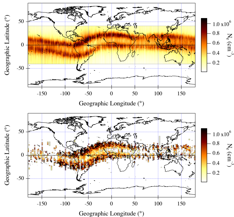
Figure 1. Top panel: Global accumulated plot of N_e values as recorded on board Swarm A from April 2014 to 31 January 2016, for Kp \leq 3 and between 18:00 and 24:00 LT. Bottom panel: Accumulated plot of the subset of N_e values corresponding to IBI = 1 and BF = 1 , and therefore to the presence of plasma bubbles, over the same time interval considered in the top panel.
